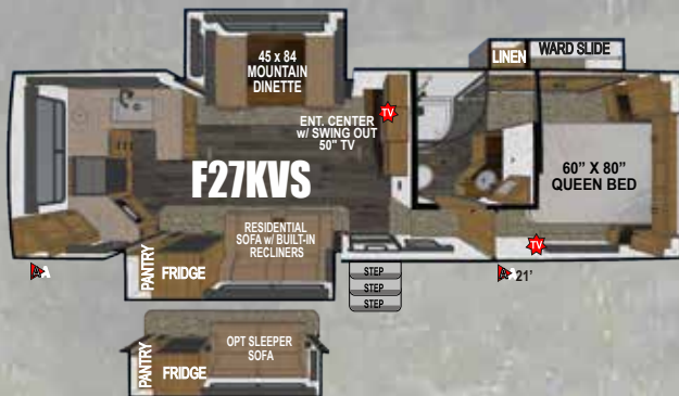
DRY WEIGHT: 9995 ~ FLOOR LENGTH: 29'
