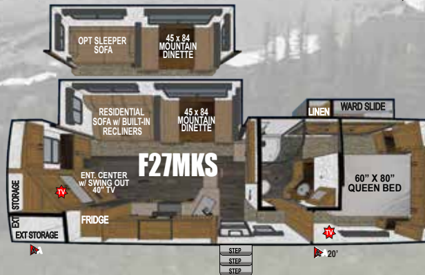
DRY WEIGHT: 9875 ~ FLOOR LENGTH: 29'
